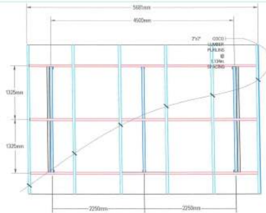
ROOF FRAMING PLAN SCALE 1/8" = 1'-0"
