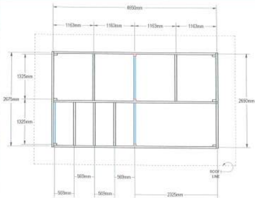
PLAN SCALE 1/8" = 1'-0"
