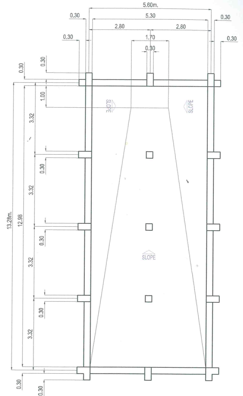
BOTTOM FLOOR PLAN
