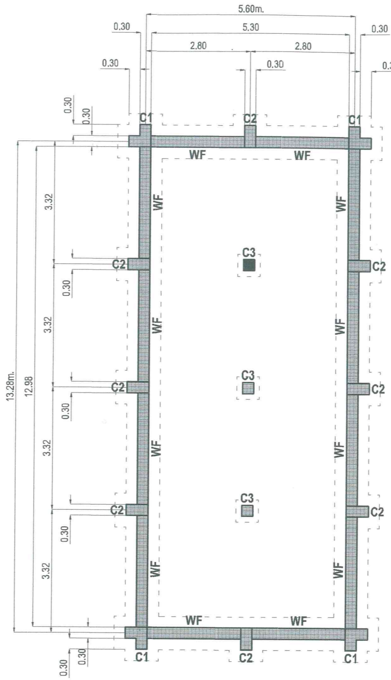
FOUNDATION PLAN
