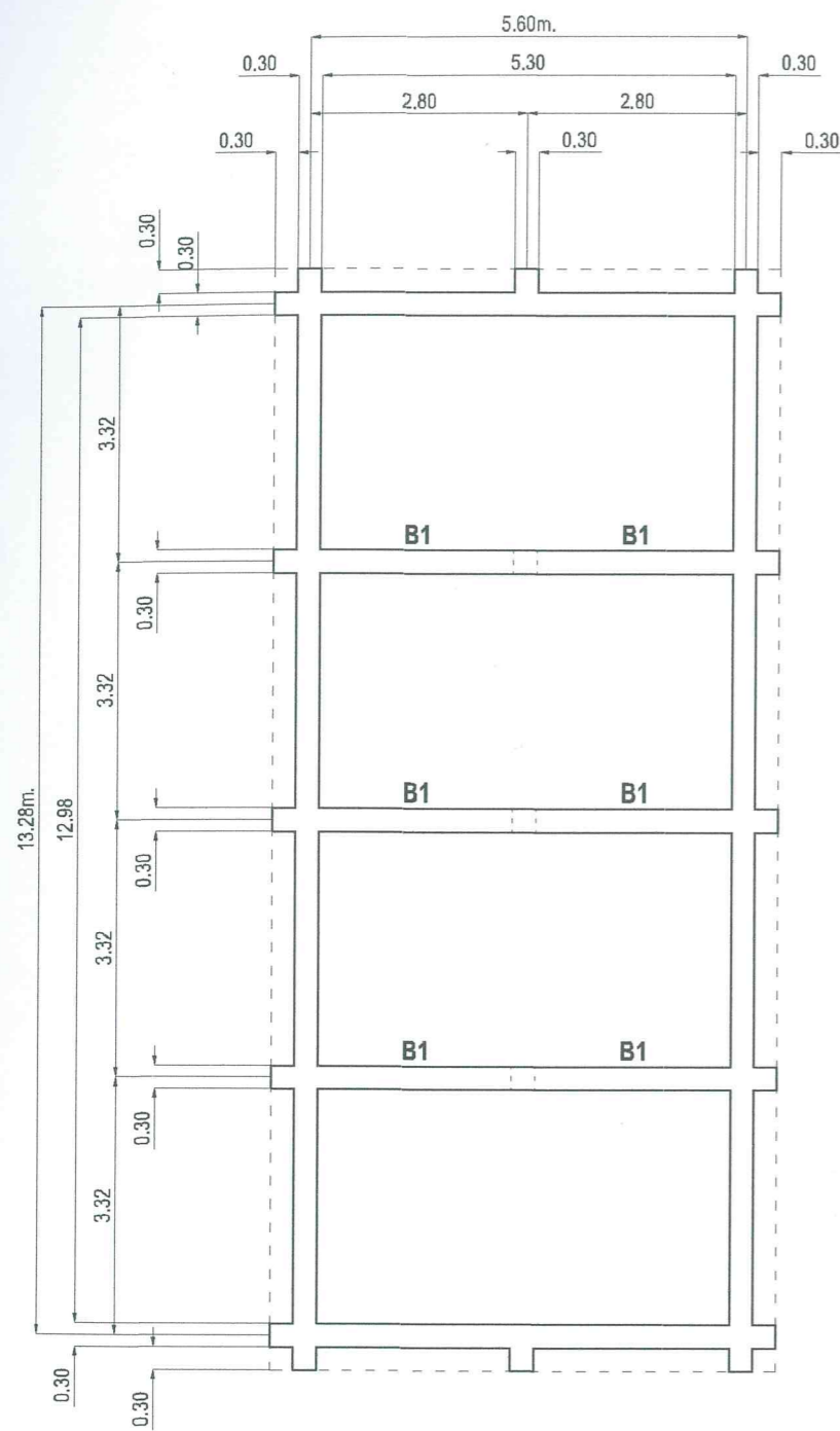
TOP FLOOR FRAMING PLAN
