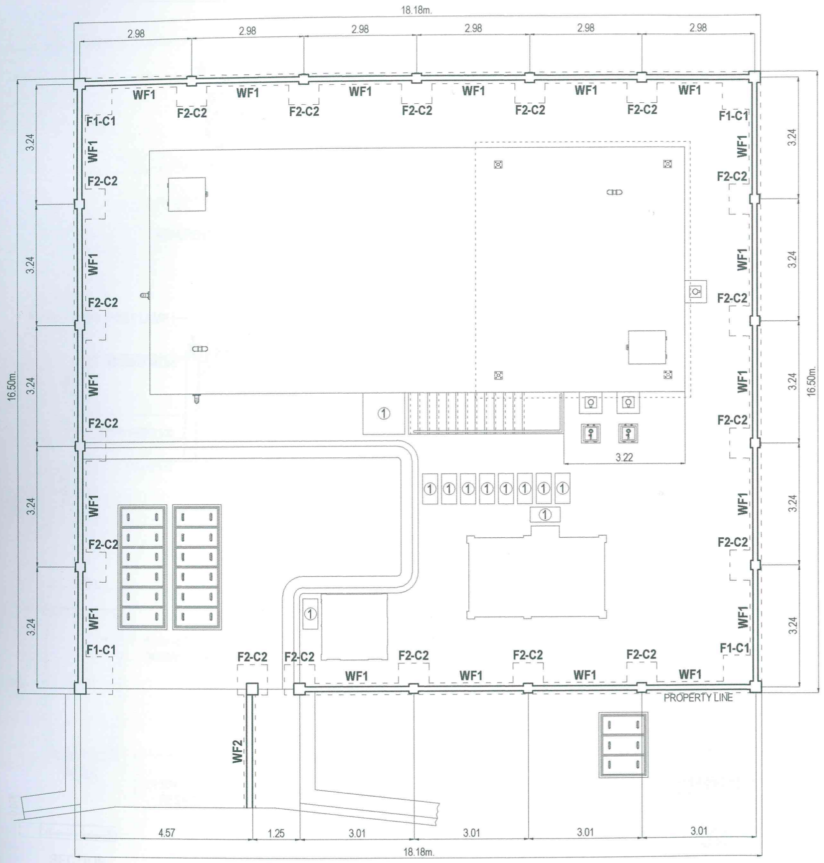
PROP. FOUNDATION PLAN OF FENCE, BANDERA SCALE: 1:100M.
