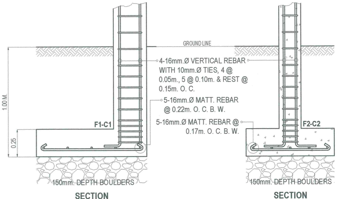
DETAIL OF COLUMN & FOOTING SCALE: 1:20 M.
