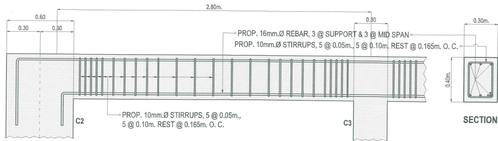
DETAIL OF BEAM 1 (B1)
