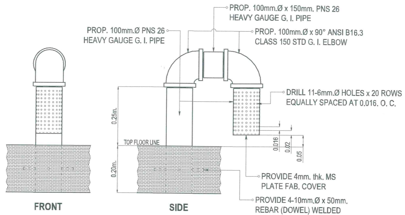
DETAIL OF AIR VENT
